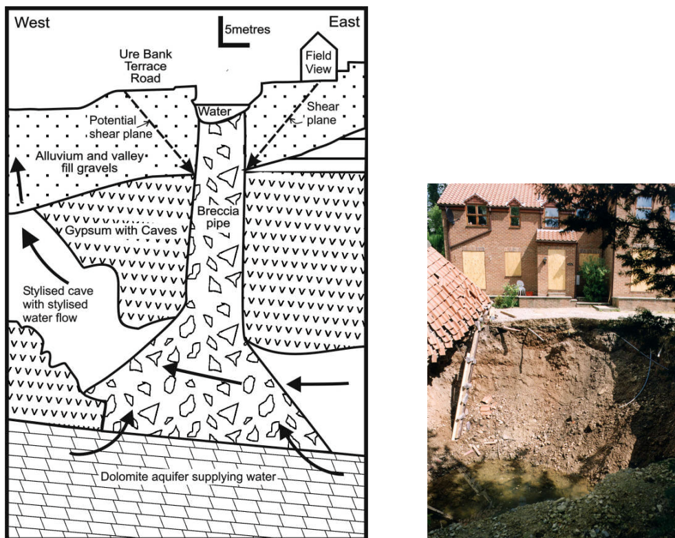
Figure 11. Schematic cross section and photograph of the Ure Bank Terrace collapse in early May 1997.
