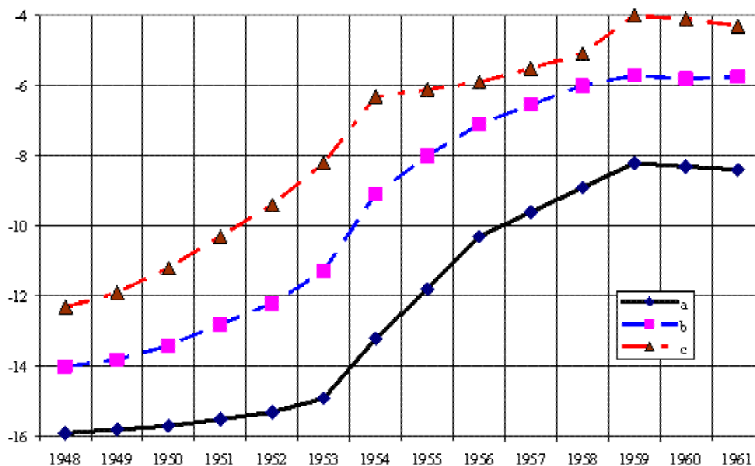
Figure 1. Changes in groundwater levels, at Novochoerkassk, from 1948 to 1961 at: a) the southern part of the city; b) the central part of the city and c) the electrode factory. The horizontal axis represents time in years and the vertical axis shows groundwater depths in metres below ground level.
