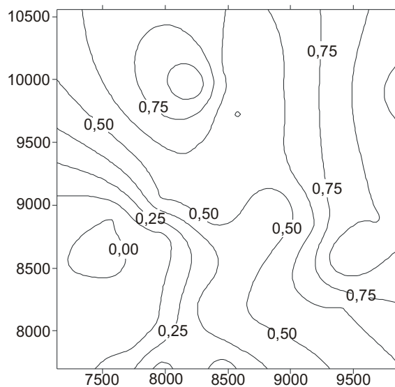
Figure 5. Schematic map to show the changes in liquidity index during flooding for the ground in the Eastern microdistrict of Novochoerkassk.
