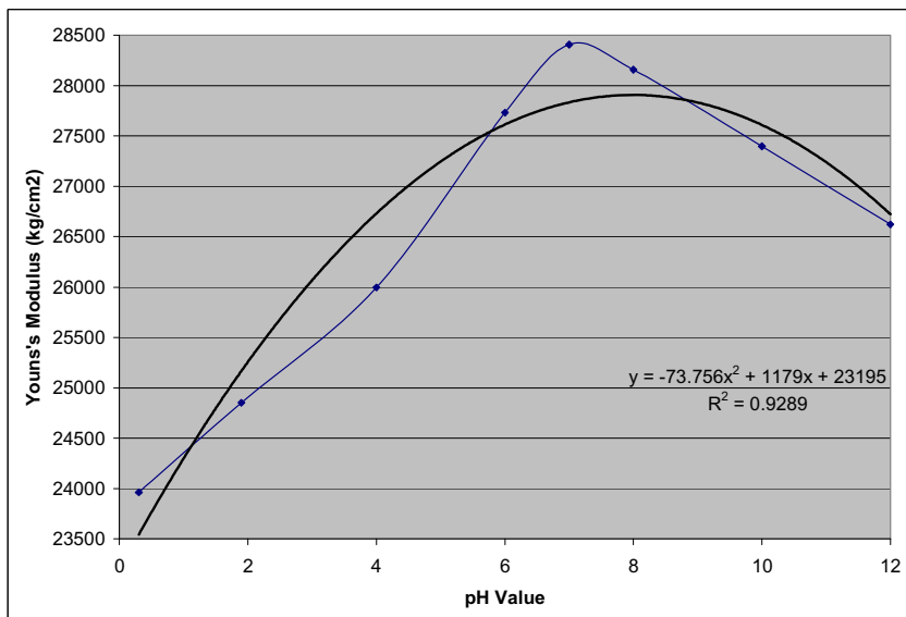
Figure 7. Relation between pH and Young's modulus.
