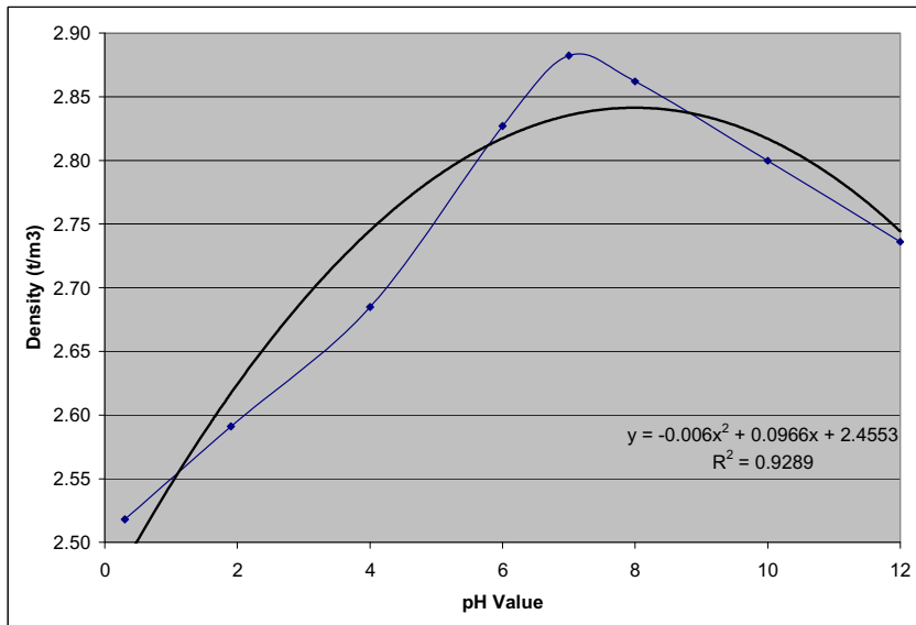
Figure 6. Relation between pH and density.
