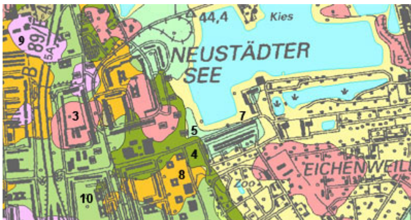
Figure 6. Section of the subsurface map from the engineering geological map of the city of Magdeburg (Annotation: 3 – anthropogenic coverage, 4 – peat, peaty clay, sapropel, alluvial mud, 5 – alluvial clay, 6 – loess and loess loam, 7 – valley sand, gravel, pebbles and boulders, 8 – melt-water sand, 9 – marly till and glacial drift, 10 – Rupel clay, 11 – greensand)
