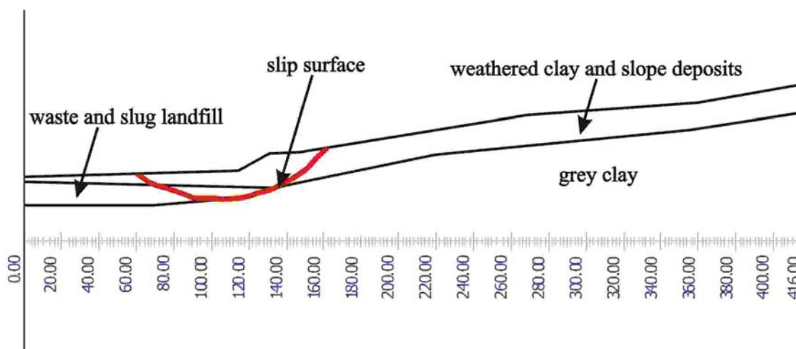
Figure 4. The model and the circular slip surface by using Geo4 (factor of safety n = 1.7 )
