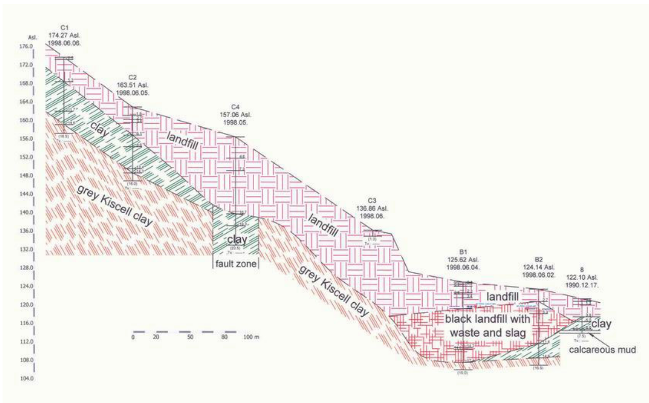
Figure 3. The geological profile of the analysed slope showing the location of drillings (borehole data from FÓMTERV, 1998)
