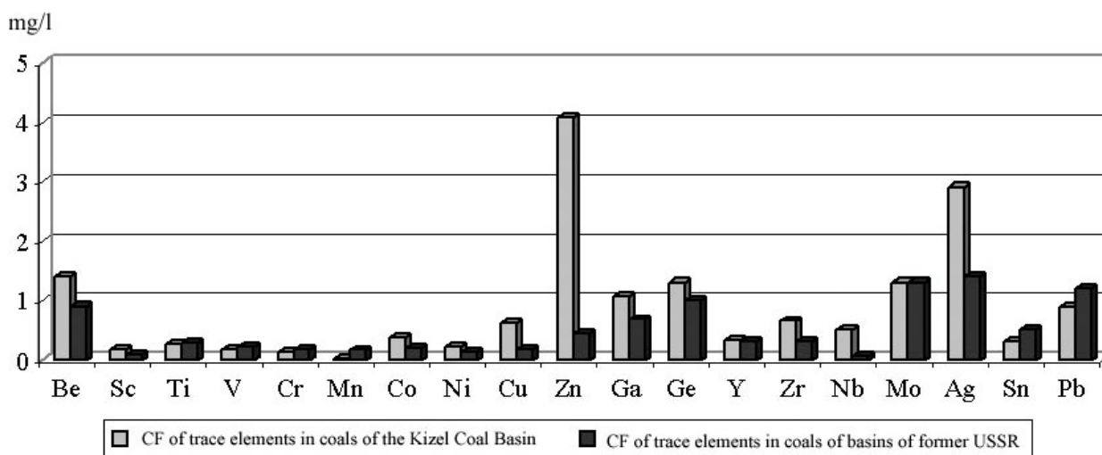
Figure 1. Coefficient factors (CF) of trace elements in coals of the Kizel Coal Basin and coals of basins of former USSR (Kler et al. 1988)
