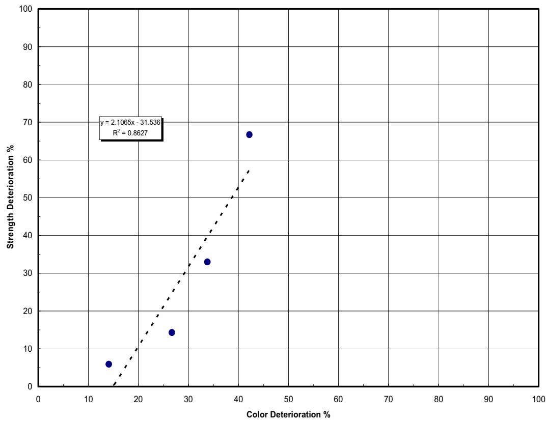
Figure 3. The relationship between color deterioration and strength deterioration in the laboratory stone samples
