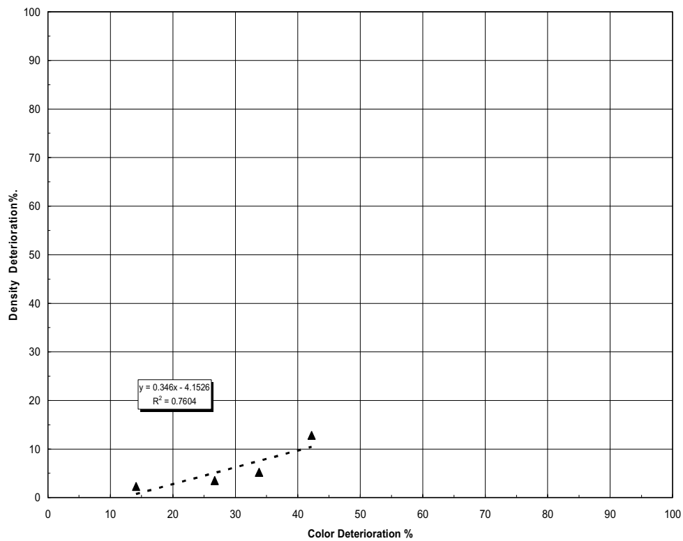
Figure 2. The relationship between color deterioration and density deterioration in the laboratory stone samples
