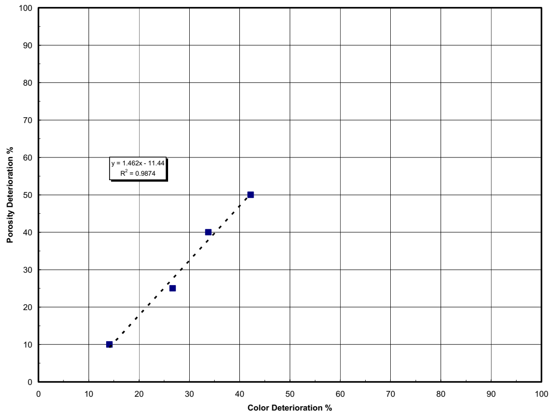
Figure 4. The relationship between color deterioration and porosity deterioration in the laboratory stone samples
