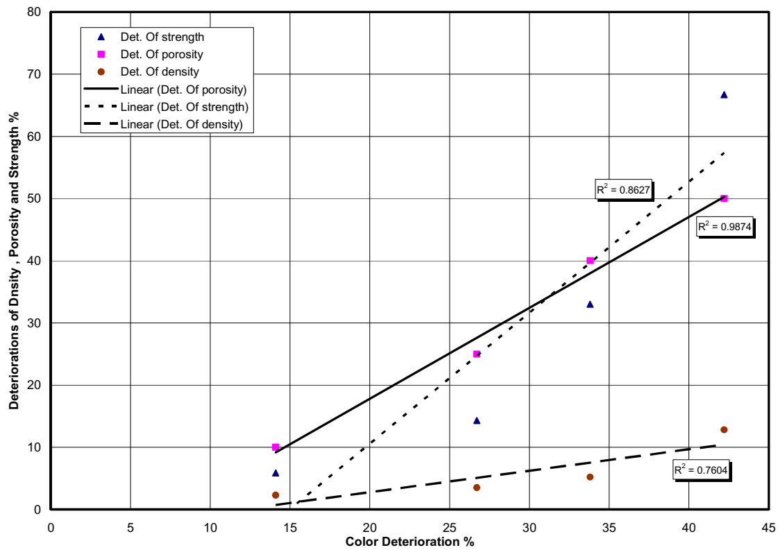
Figure 5. Relationship between color deterioration and the deterioration in density, porosity and strength of the laboratory stone samples
